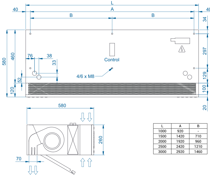
Horizontal installation
