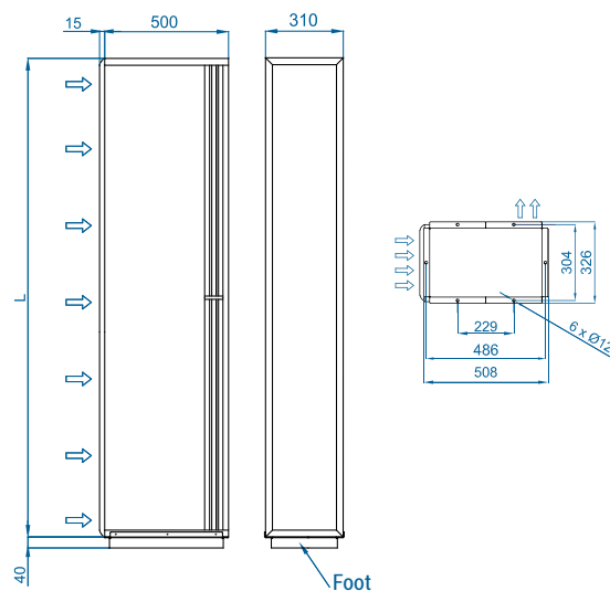
Vertical installation
